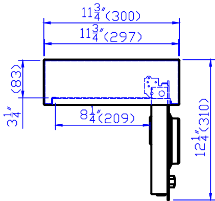
Top view door open
